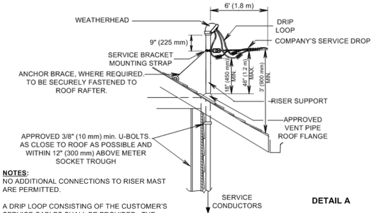
Figure 4.2.4.3-1 Overhead Service Attachment and Riser Mast Requirements
