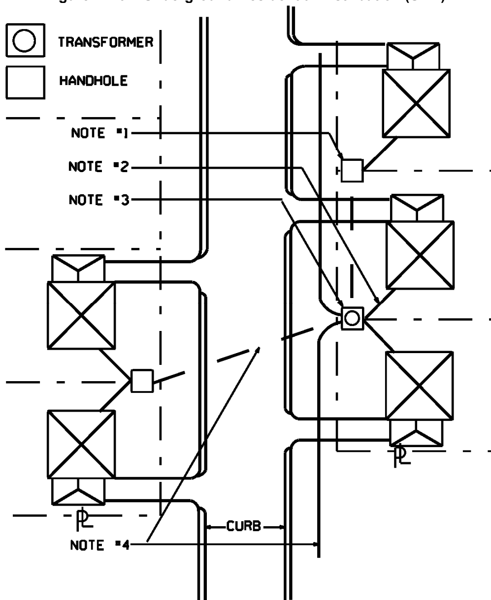
Figure 4.4.6-1 Underground Residential Distribution (URD)
