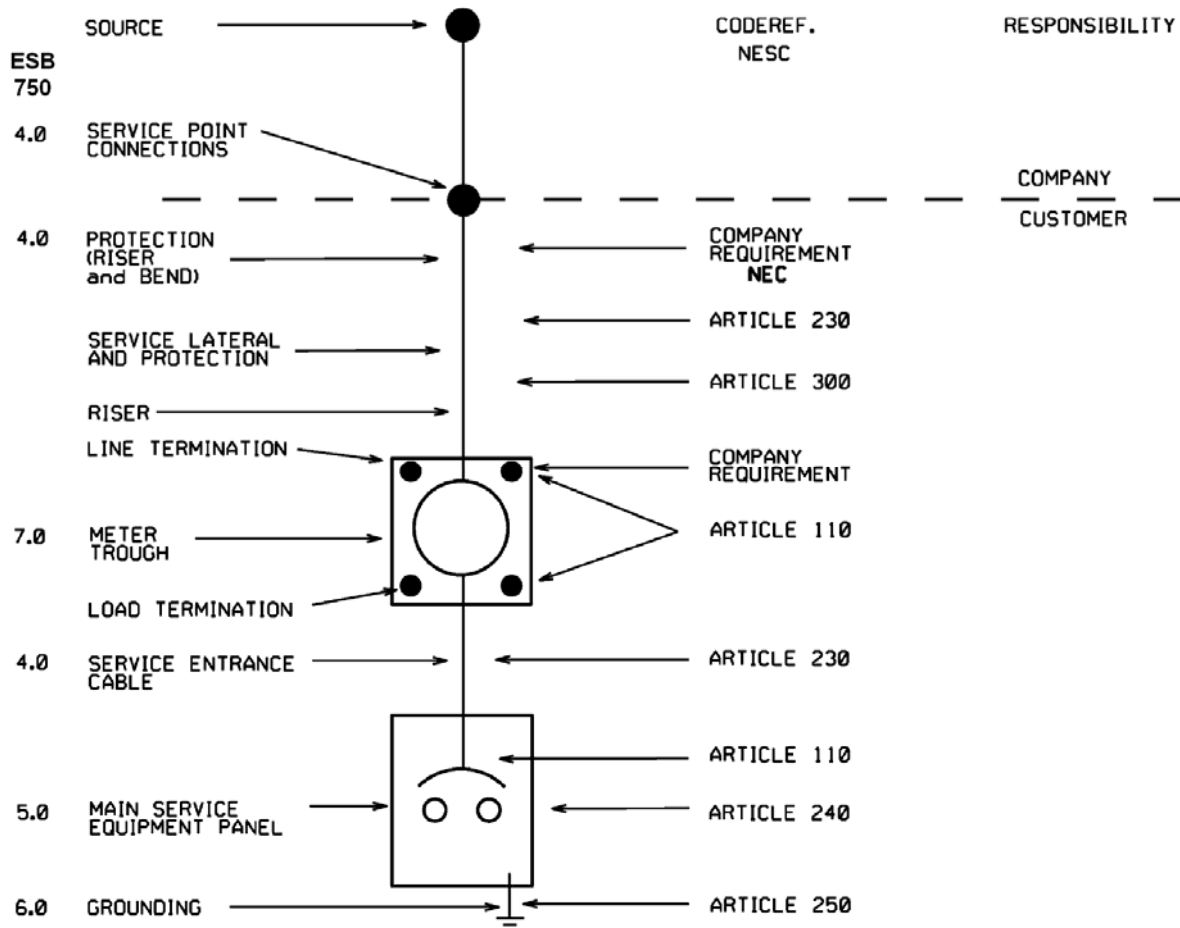
Figure 4.4.1-1 Typical Underground Service Installation under 600V (Excluding Network Services)
