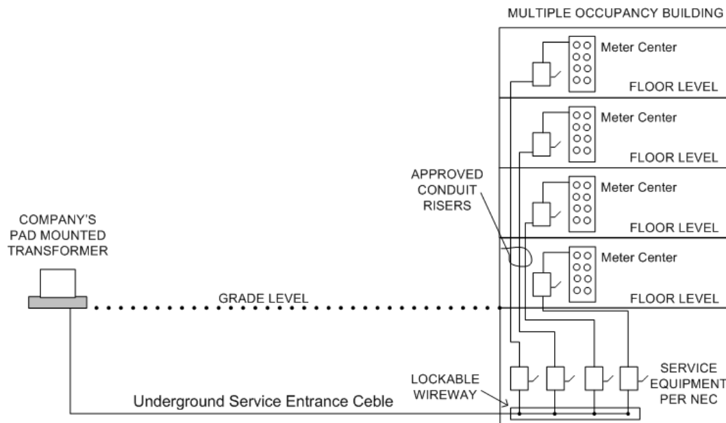
Figure 4.4.7.3-1 Typical Service to Multiple Occupancy Building
