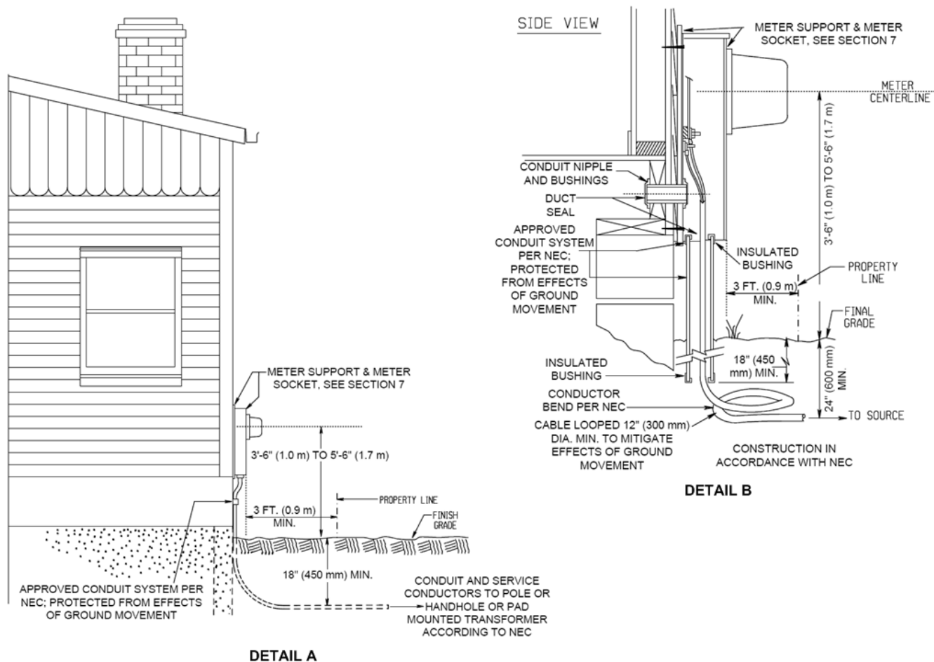
Figure 4.4.6-2 Underground Secondary Service Residential Meter Connection – Conduit or Direct Buried
