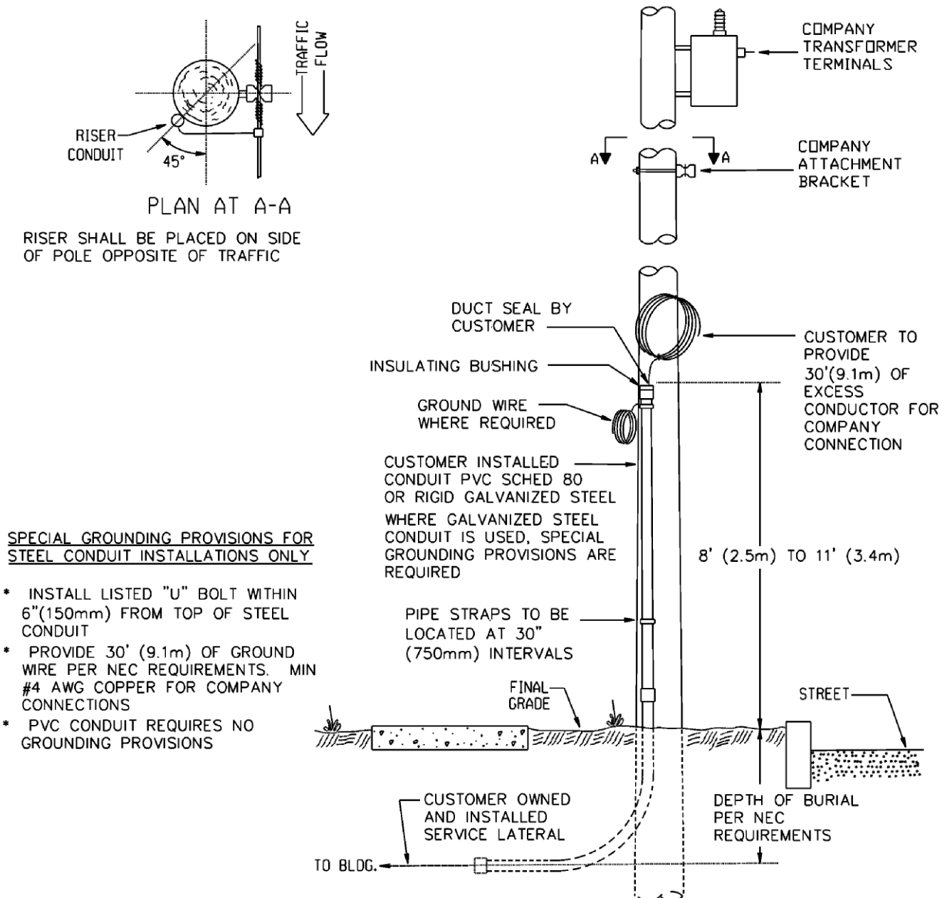
Figure 4.4.4.2-1 Underground Secondary Service Riser Pole Detail
